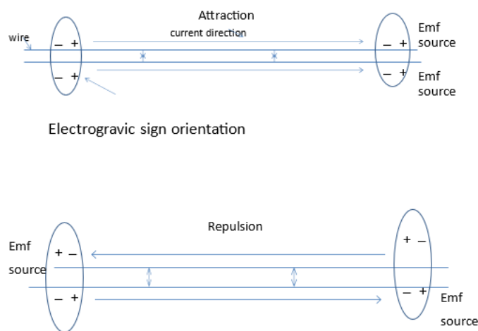
Fig 2. Shows how orientation of gravitational charge, amplified in parallel current-carrying wires as electromagnetism, follows exactly the rule of attraction and repulsion for secondary charge
